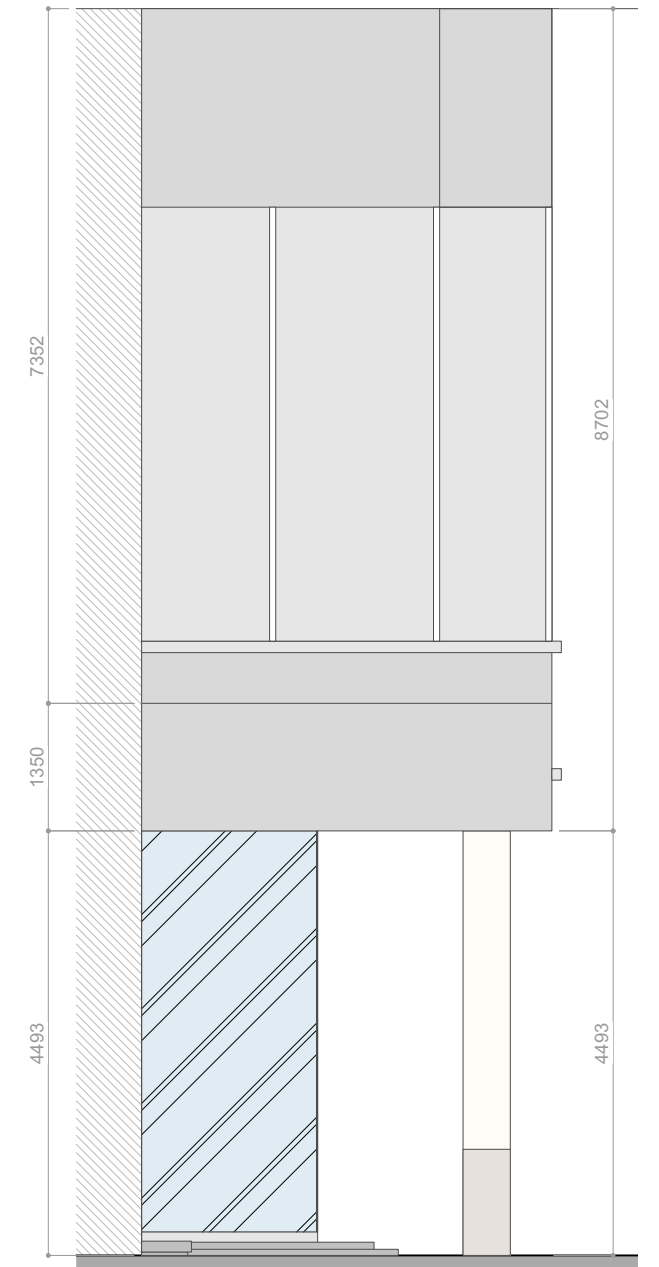
C elevation
